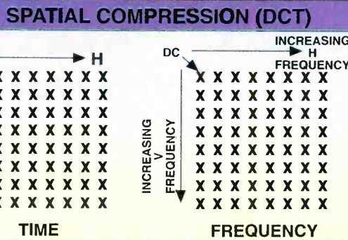
Figure 2. For spatial compression, the discrete cosine transform (DCT) is used to convert time-based data to frequency-based data.
