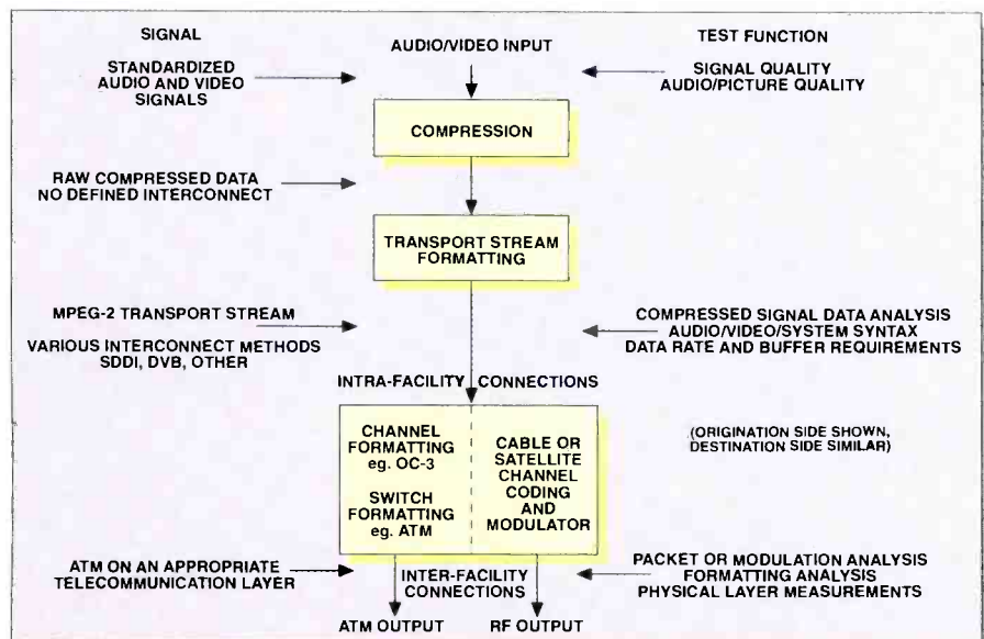
Figure 4. Signals and test functions used at various TV/telecommunication layers.
