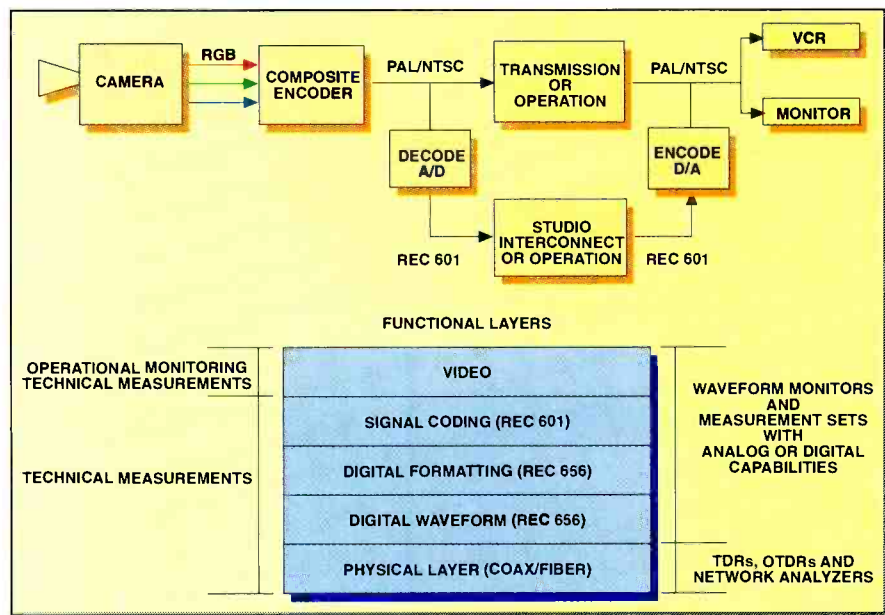
Figure 1. Block diagram of a typical uncompressed video system, along with a depiction of the layers involved and the test equipment used.
