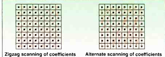
Figure 4. To improve the overall compression, coefficients are scanned using one of two methods. In this manner, the data is formatted for optimum run-length encoding.
